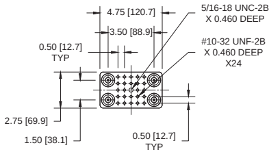
MOUNTING PLATE TOP VIEW
