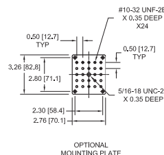
OPTIONAL MOUNTING PLATE
