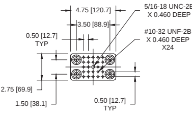
MOUNTING PLATE TOP VIEW
