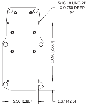
BENCH MOUNTING HOLES BOTTOM VIEW
